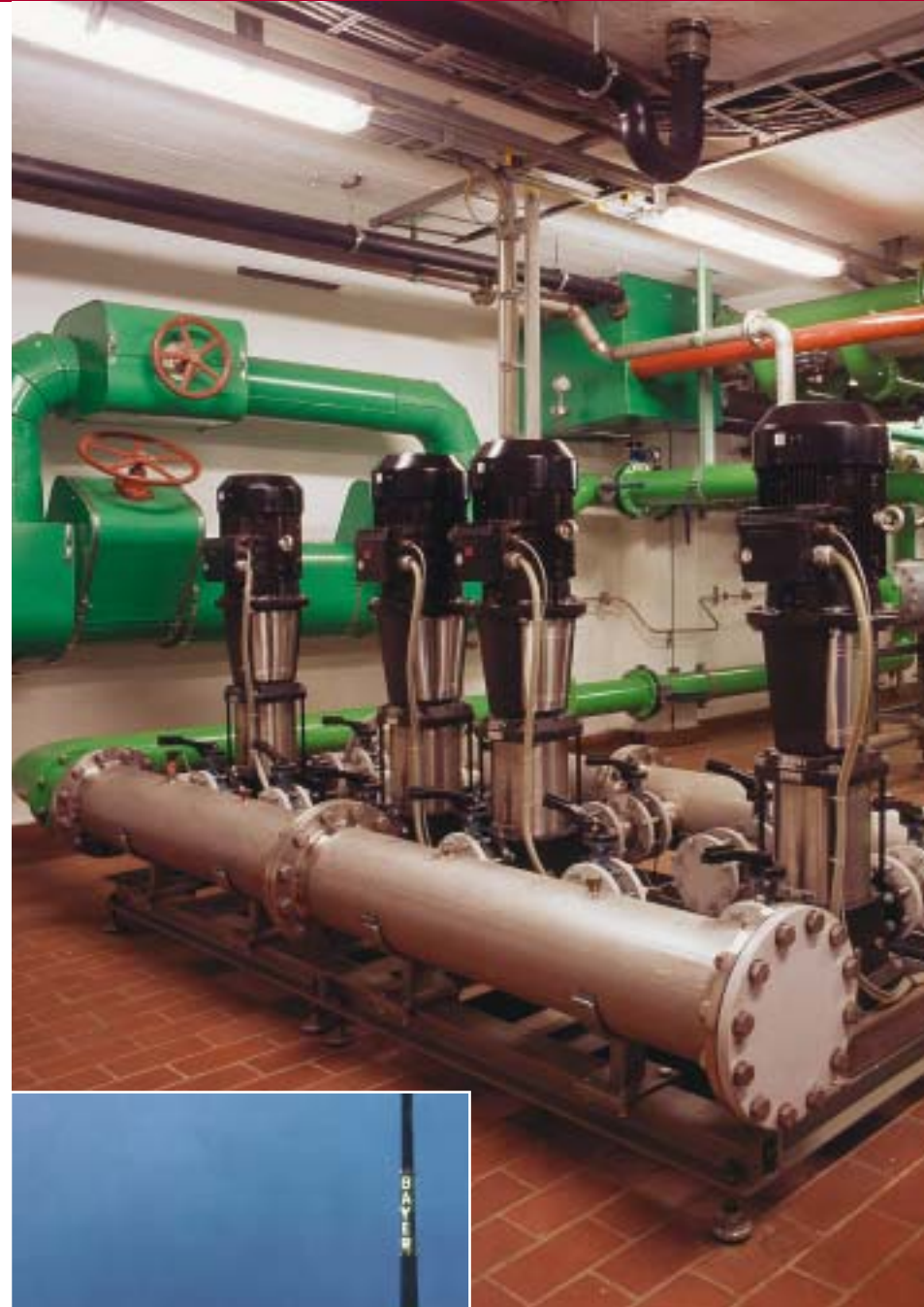
A Grundfos Hydro 2000 booster installed in the Bayer production plant, Germany, where it is boosting water pressure for the production of pharmaceuticals.
