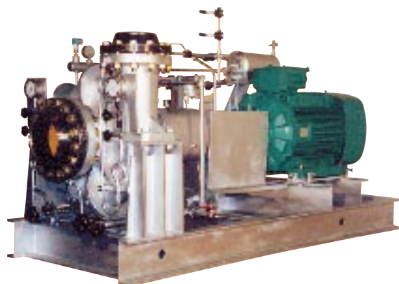
Pompe process haute température High temperature process pump
