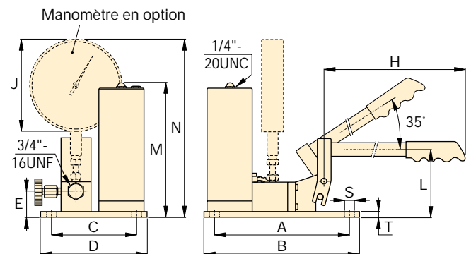
11-100, 11-400
