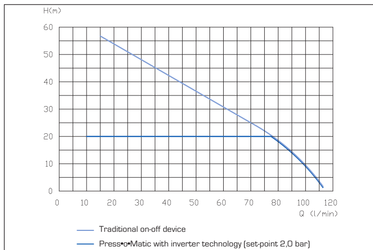
PRESSURE FLOW RATE DIAGRAM (ELECTRIC PUMP 1,5 HP)
