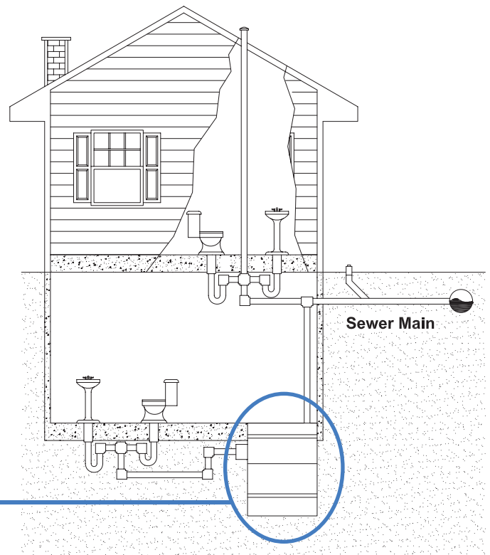
TYPICAL SEWAGE SYSTEM
