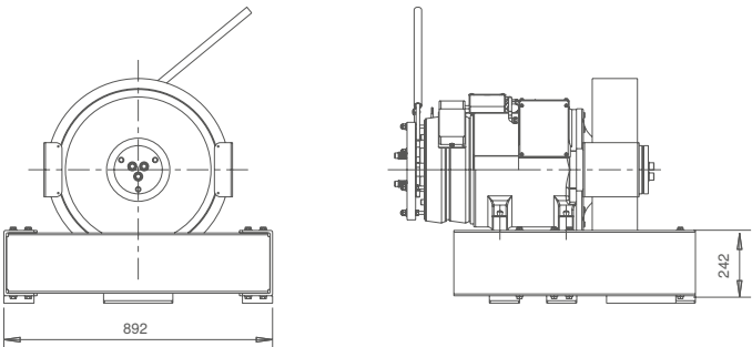
Dimensions mm
