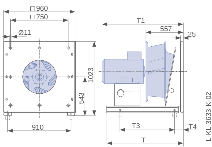
Dimensions mm
