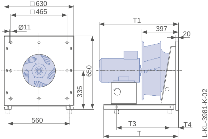
Dimensions mm
