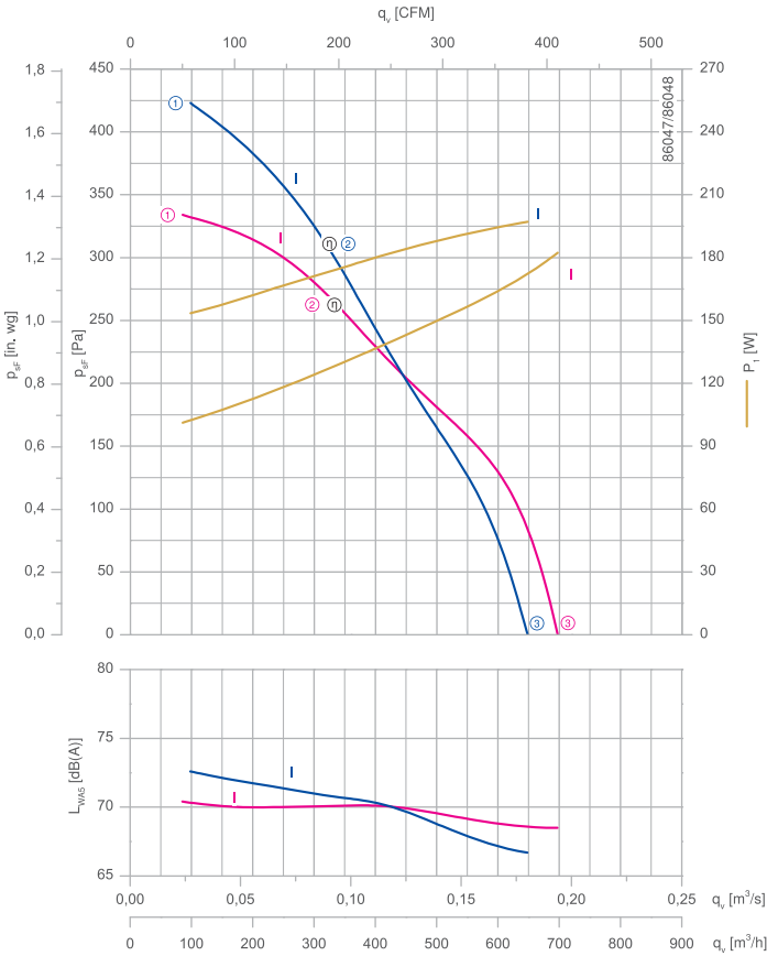
Characteristic curve
