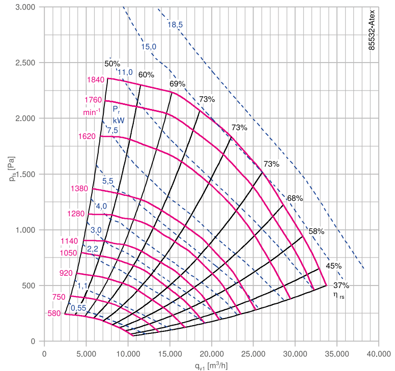
Characteristic curve
