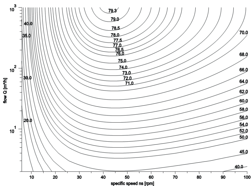
MEI = 0.4 for Multistage Vertical 2900rpm
