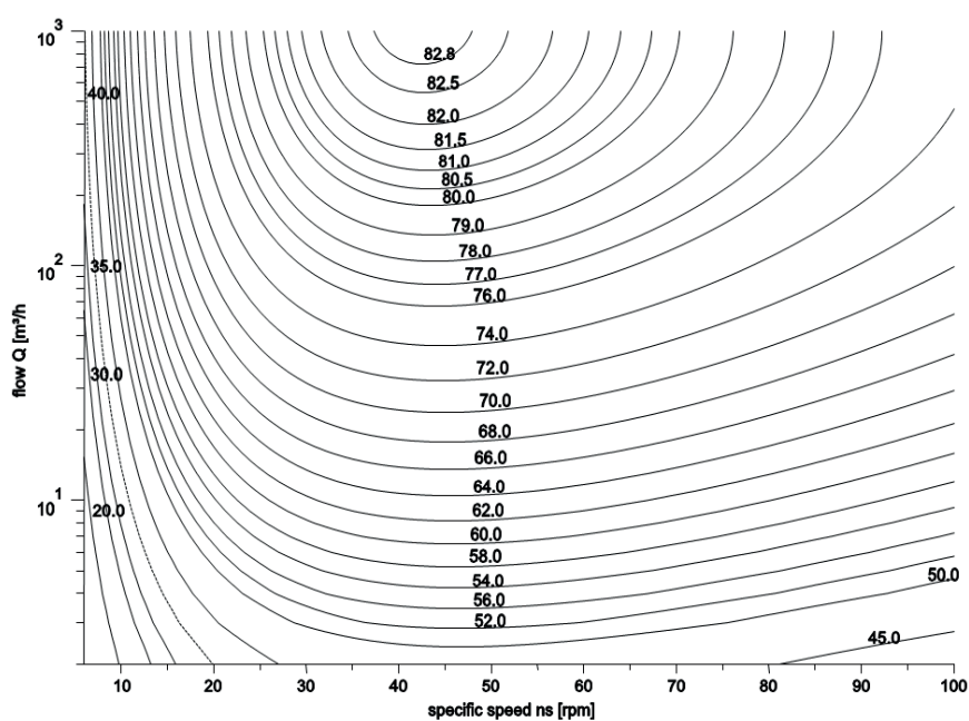
MEI=0.7 for Mutistage Vertical 2900 rpm
