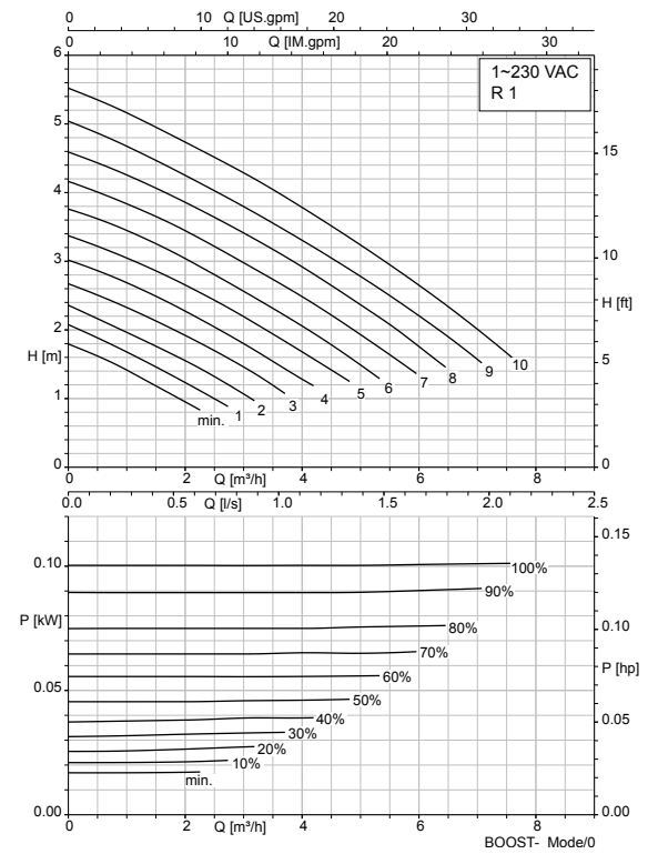
Calio 25-60, Boost
