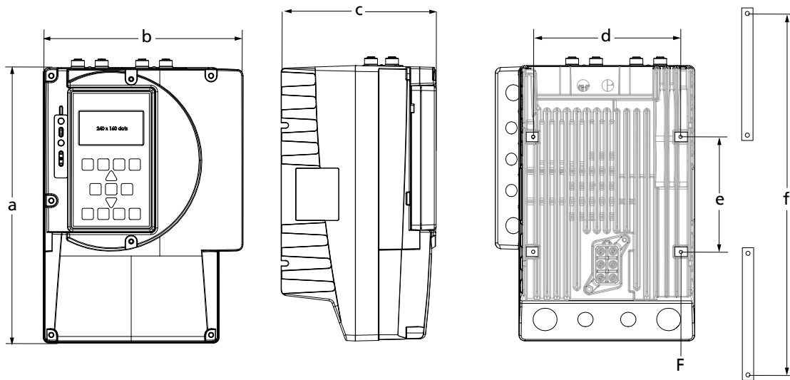
III. 4: Dimensions PumpDrive 2
