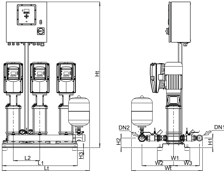
III. 10: Dimensions
