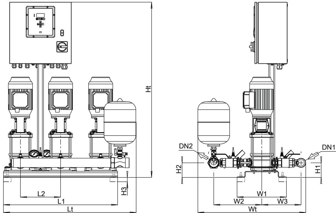
III. 3: Dimensions
