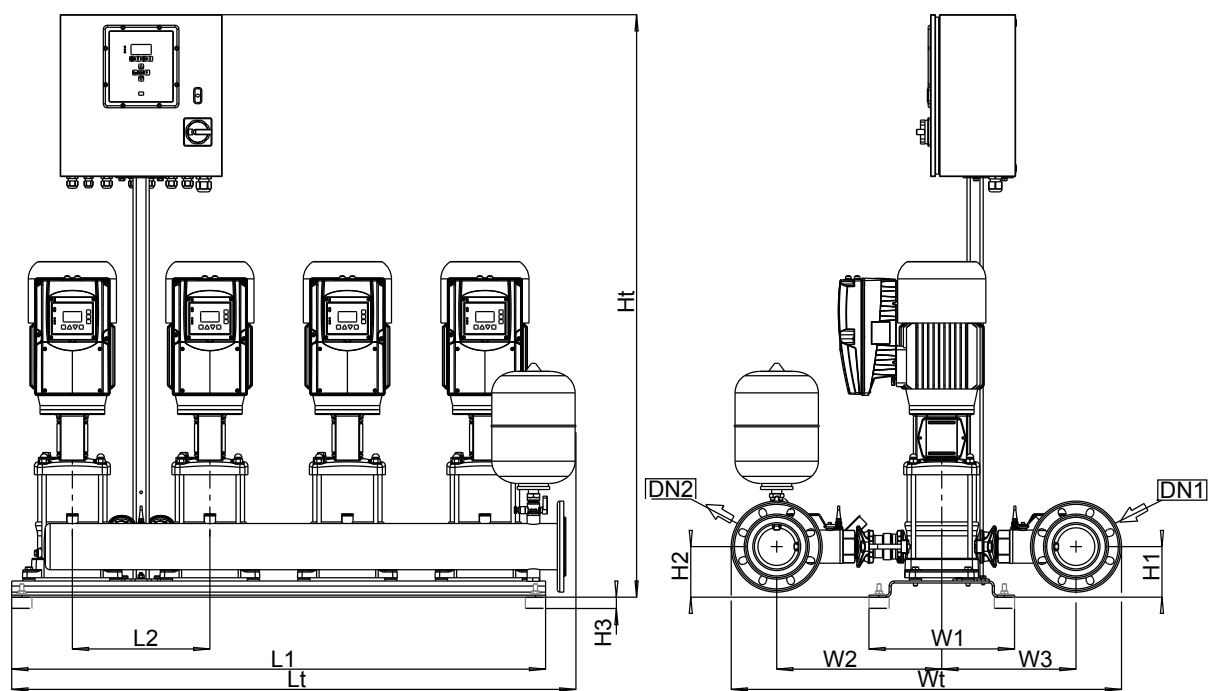
III. 13: Dimensions
