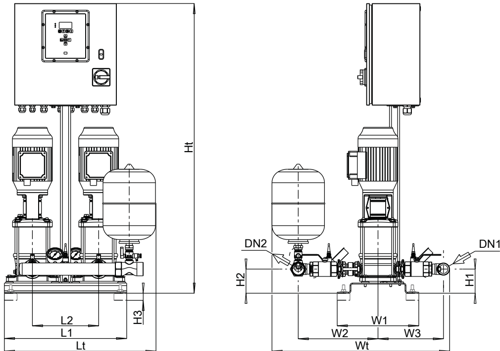
III. 2: Dimensions
