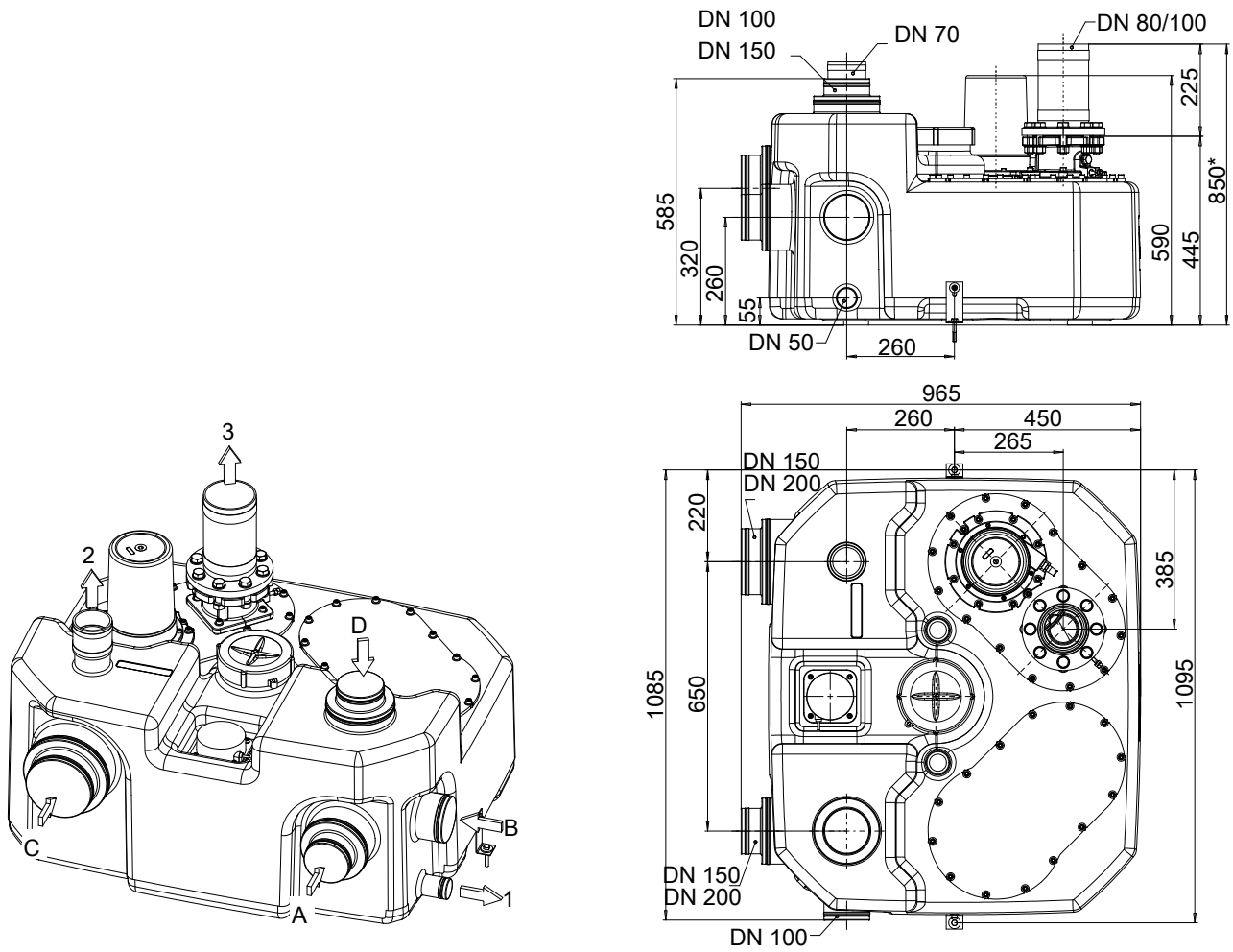
III. 6: Raccords et dimensions Compacta U (300 litres)
