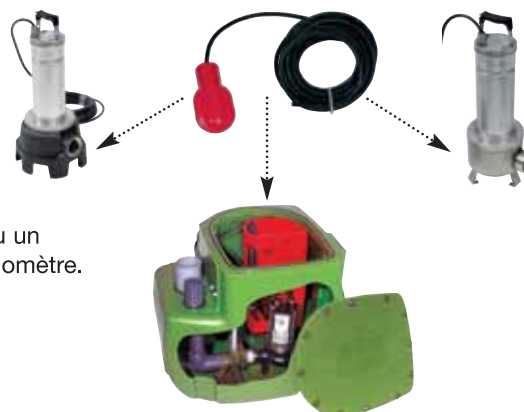
PROTEC 2 Relevage
