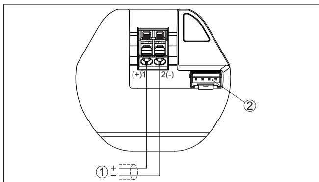
Fig. 20: Compartiment de raccordement VEGAPULS 31
