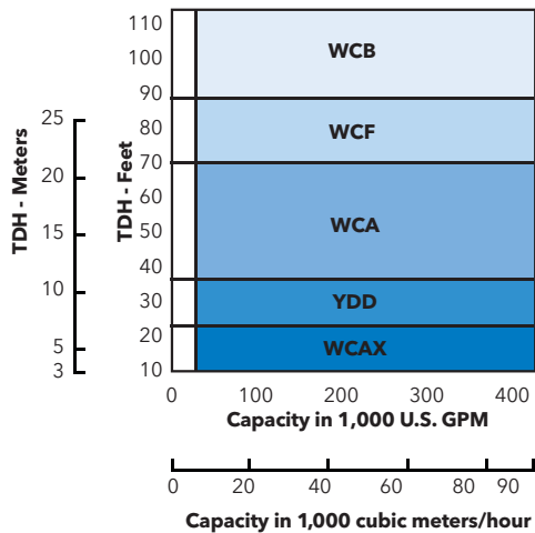
LOW TO MEDIUM HEAD PUMPS RANGE CHART
