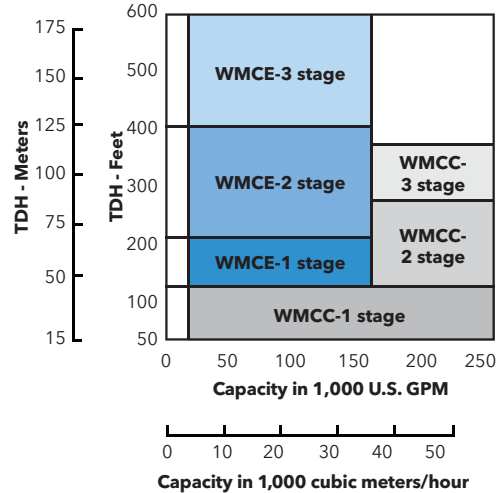
HIGH HEAD PUMPS RANGE CHART
