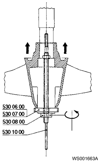
Рис. 56: P7045, P7055, P7076
