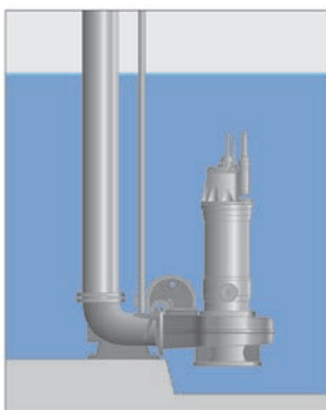
NP – For semi-permanent wet well installations: the pump is installed with twin guide bars and a discharge connection.
