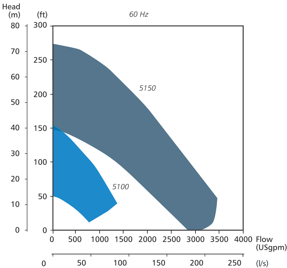
5100/5150 performance range
