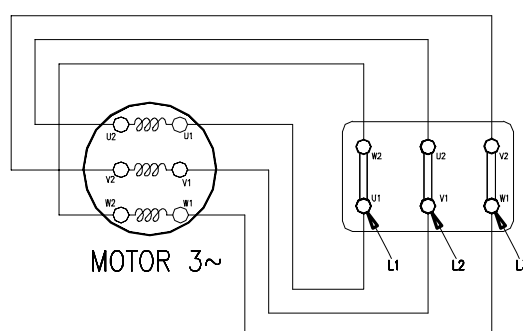
DELTA CONNECTION
