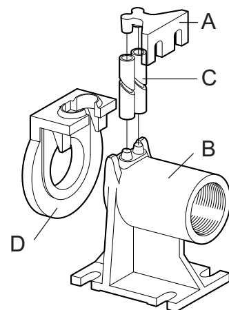
Fig. 7 Foot pedestal
