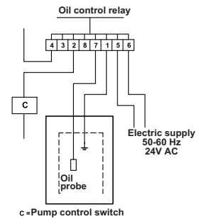
Fig. 14 Oil level probe connection
