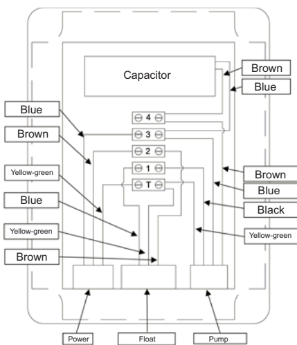
Fig. 8 Wiring diagrams for a single-phase pump with and without float.
