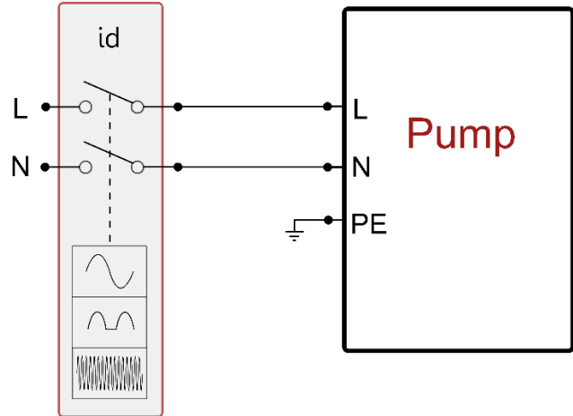
Fig 11 example of single-phase installation
