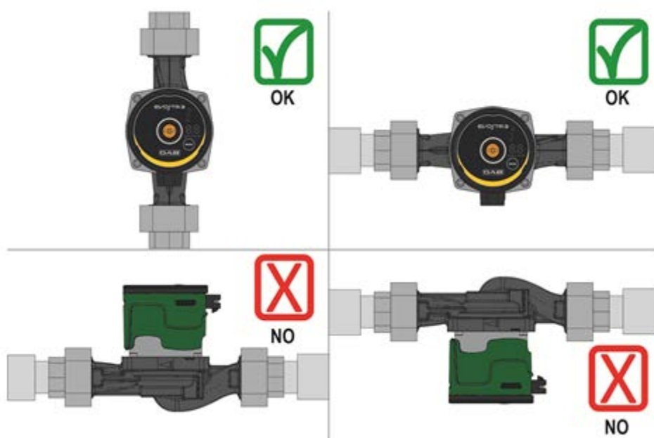
Fig. 3: Monteringsposition
