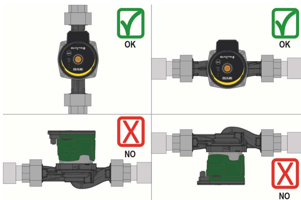
Abb. 12: Montageposition
