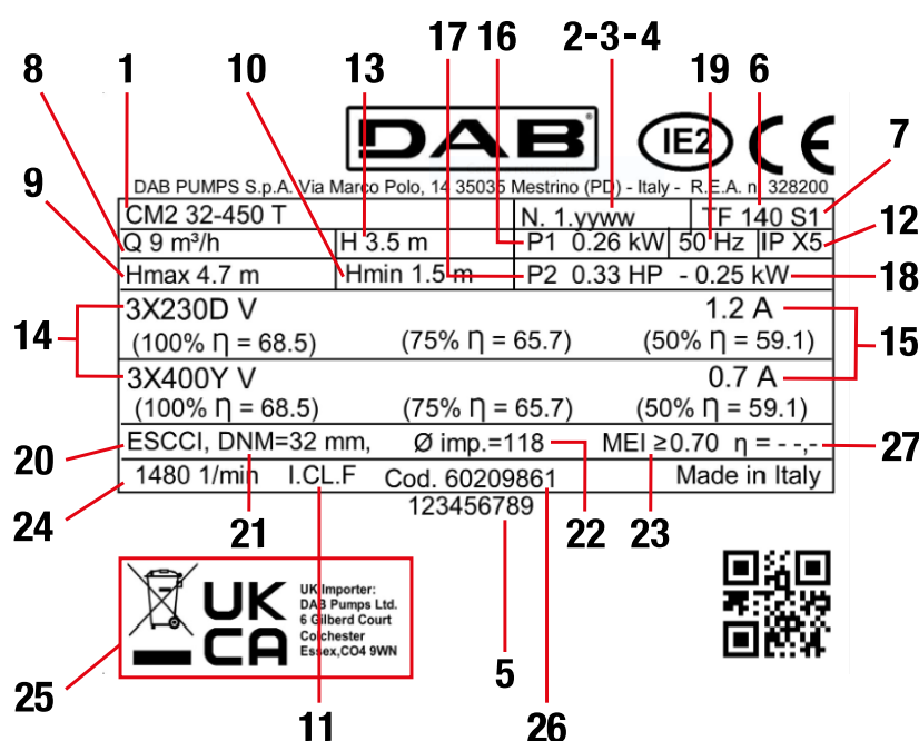
Fig.1 Data plate
