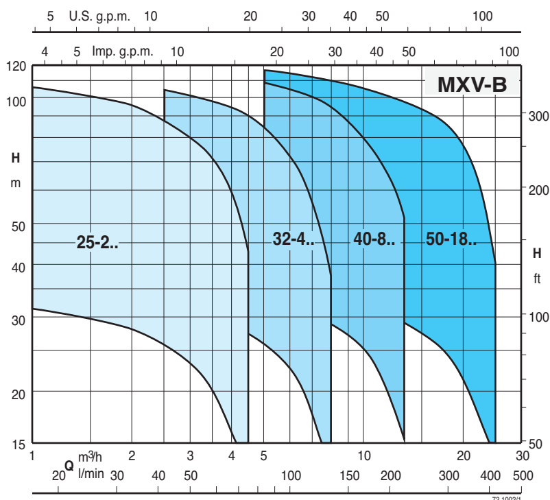
Coverage chart n \approx 2900 rpm
