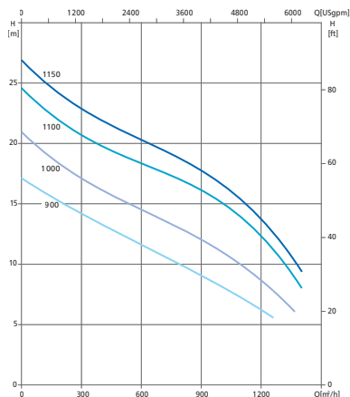
Performance Curves accor. to UNI 9906
