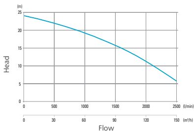
Performance curve
