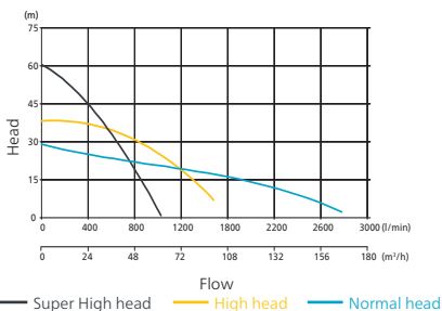
Performance curve
