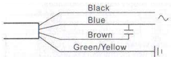
Figure 2: Single-phase wiring diagram
