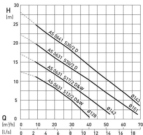
AS 0631 and 0641
