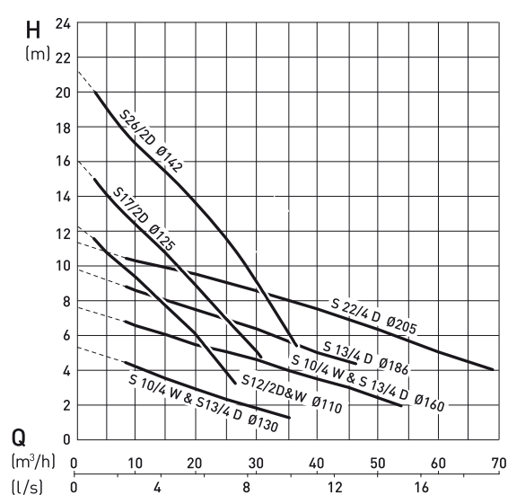
AS 0530, 0630 and 0830
