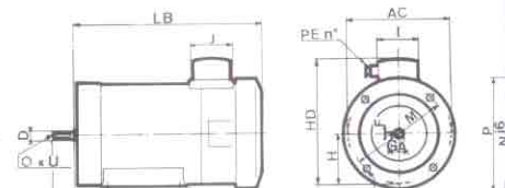
A TROUS LISSES
