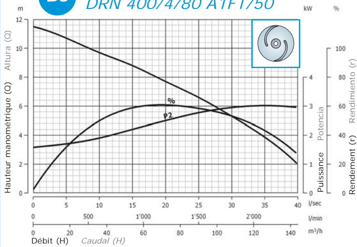
B5 DRN 400/4/80 A1FT/50
