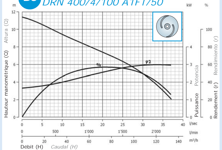
B6 DRN 400/4/100 A1FT/50
