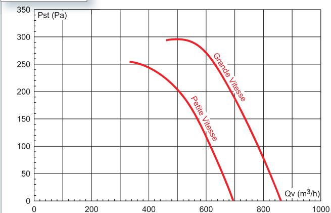
THC-800 Insufflation
