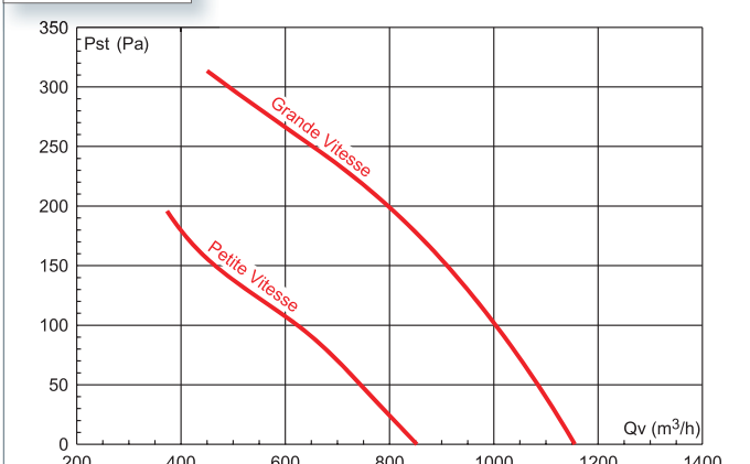
THC-1300 Insufflation
