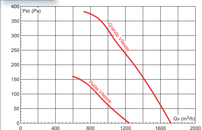
THC-2000 Insufflation
