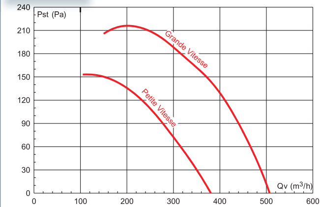
THC-500/160 Insufflation
