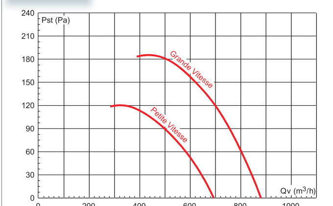
THC-800N Insufflation
