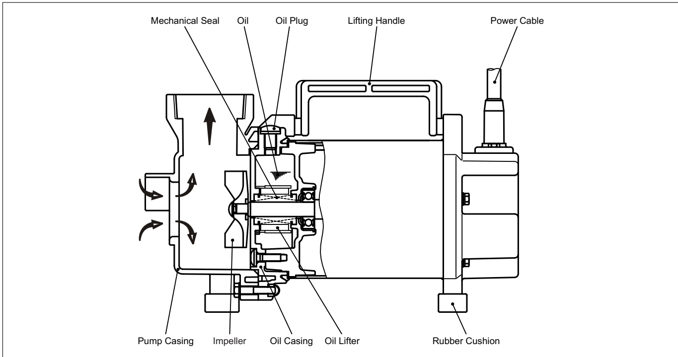
FIGURE 1.1 PARTS LISTING
