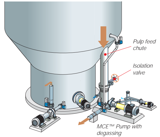
Fig. 23. MC® parallel pumping system arrangement.
