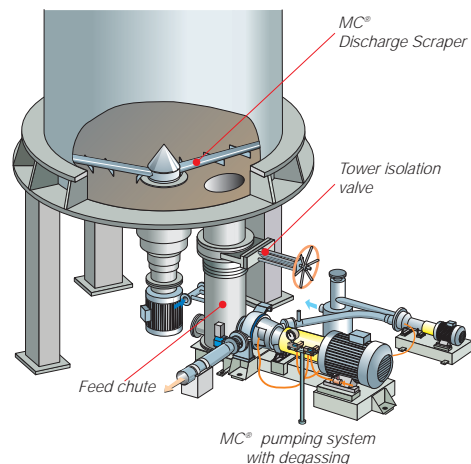
Fig. 14. MC® pumping system components in a tower discharge pumping system.
