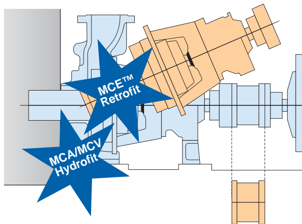
Fig. 9. MCE™ Retrofit and MCA/MCV Hydrofit.
