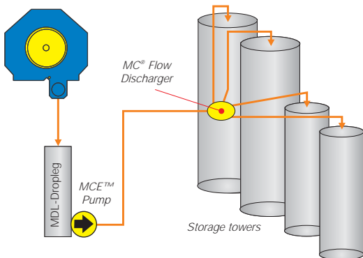
Fig. 19. MC® Flow Discharger in storage tower application.
