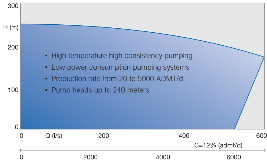
Fig. 4. MCE™ Pump series capacity range.
