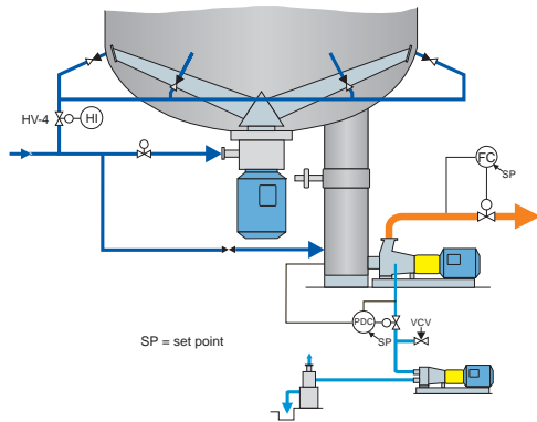
Fig. 16. Control system in MC® tower discharge installation.
