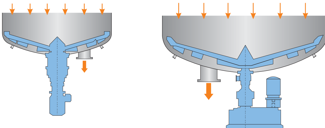
Fig. 15. MC® Discharge Scraper constructions.
