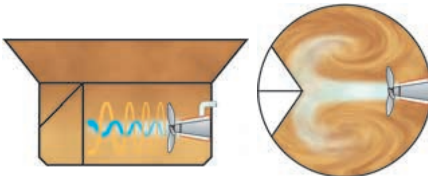
Fig. 4. Flow divider Plough keeps the agitation only in the bottom zone of an MC tower. The small agitated volume needs less energy than a bigger volume. Also, consistency control of a small volume is quicker than the control of a big volume. Dilco feeds dilution water into the center of the propeller.
