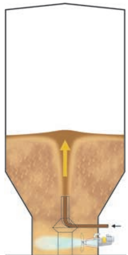
Fig. 6. The Vulca method fills the tower so that inflow does not mix air into the stock. The pumping energy can be adjusted according to the stock level so that with a low level, the speed of the pump is lower than with a high level.
