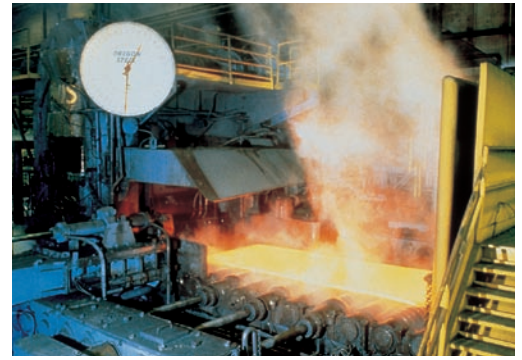
Accurately measuring temperature of slabs, billets, or blooms on a hot rolling mill ensures product uniformity.
