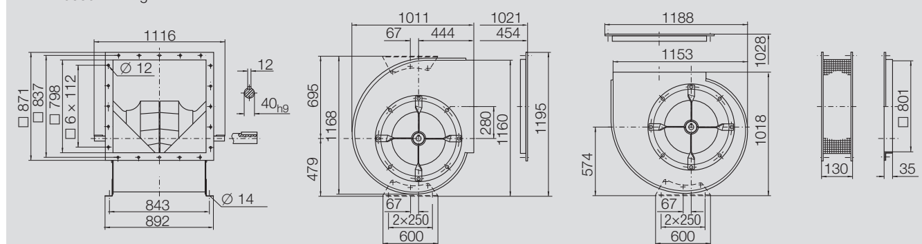
RZR 12-0630 132 kg
