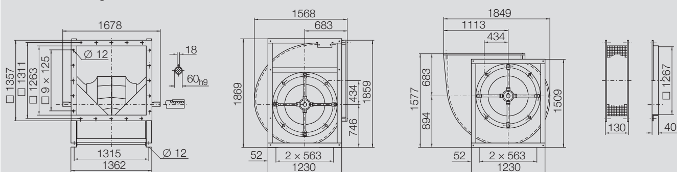
RZR 18-1000 471 kg
