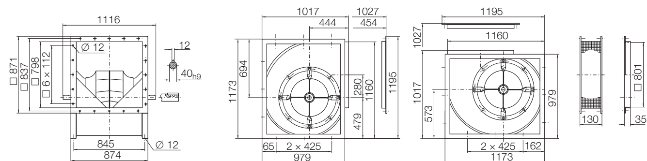
RZR 15-0630 149 kg
