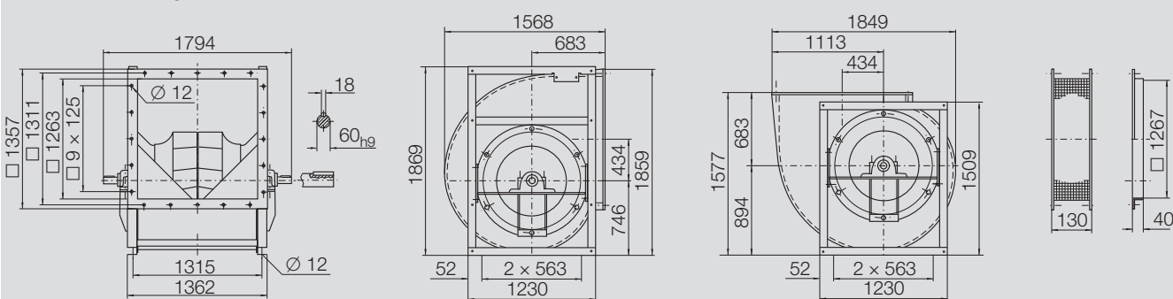
RZR 13-1000 517 kg
