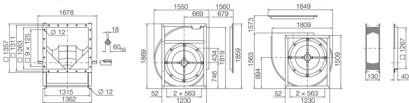
RZR 19-1000 462 kg
