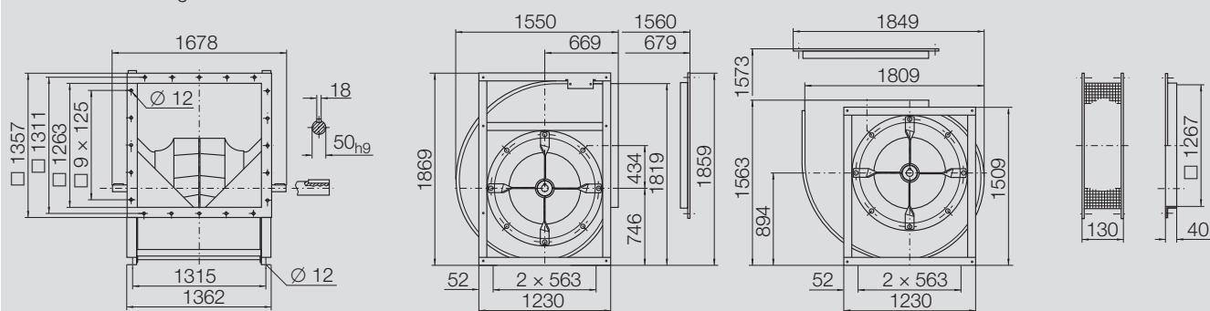
RZR 15-1000 416 kg
