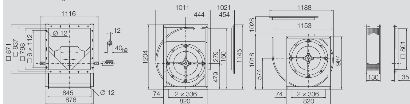
RZR 19-0630 162 kg
