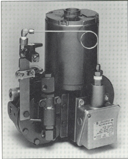
mRoy A with diaphragm rupture detection system including pressure switch.
