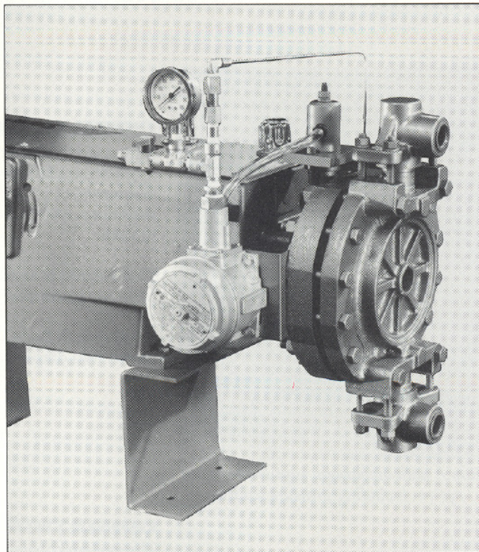
maxRoy B with diaphragm rupture detection system.
