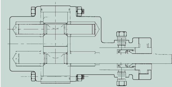
FIG.2 SINGLE MECHANICAL SEAL
