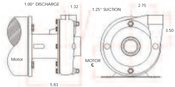
Mag-drive, Close-Coupled
