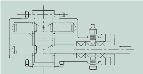
FIG.1 PACKING SEAL
