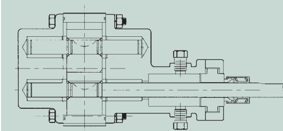
FIG.3 EXTERNAL MECHANICAL SEAL
