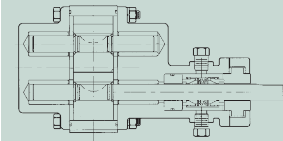
FIG.4 DOUBLE MECHANICAL SEAL
