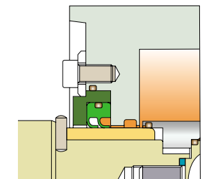
Lip Seal
