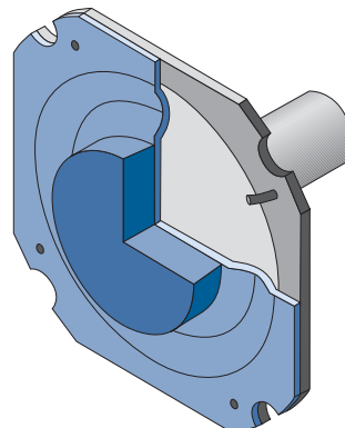
Standard double-diaphragm
