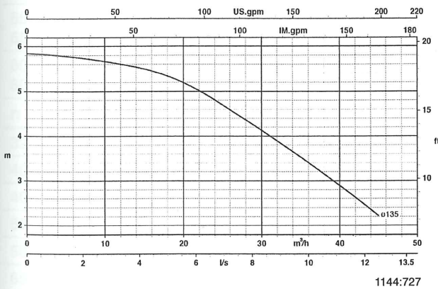
Trialine Z 80-125/034
