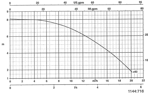
Trialine Z 40-100
