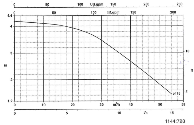
Trialine Z 65-125/034
